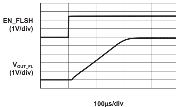
Start-Up Time (100mA Load)
