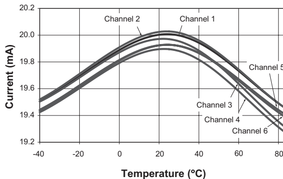
Current Matching vs. Temperature
