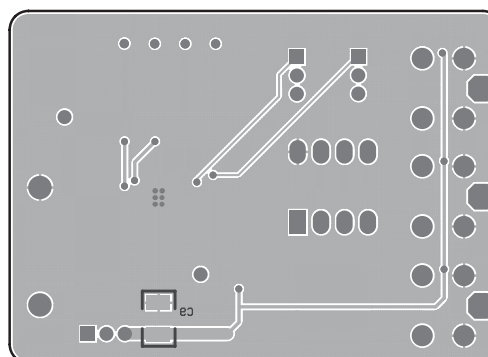
Figure 4: AAT2845 Evaluation Board Bottom Layer.
