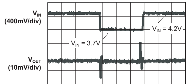
LDOB Line Transient Response (10mA Load)
