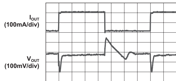
LDOB Load Transient Response
