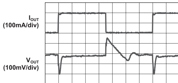
LDOA Load Transient Response
