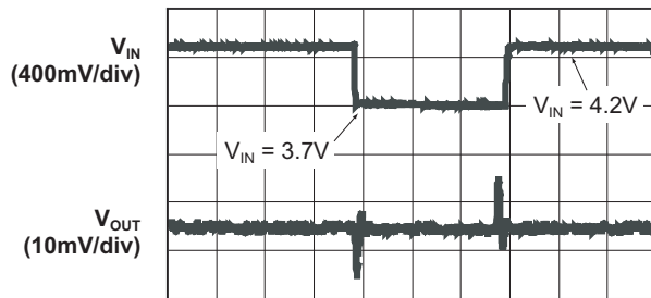
LDOA Line Transient Response (10mA Load)
