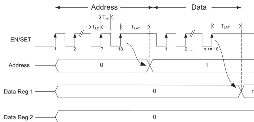
Figure 1: AS²Cwire Serial Interface Timing.
