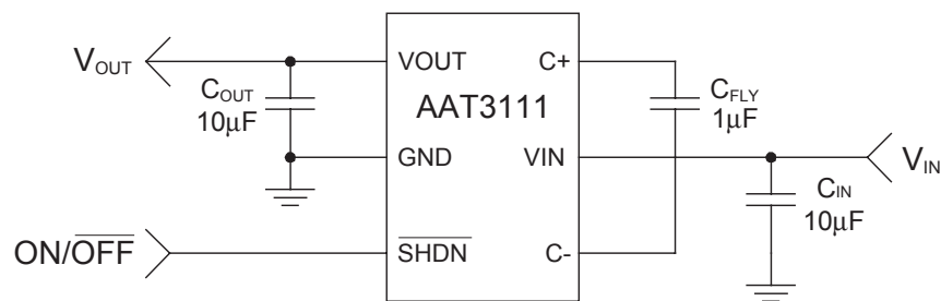
Figure 6: Typical Charge Pump Boost Converter Circuit.
