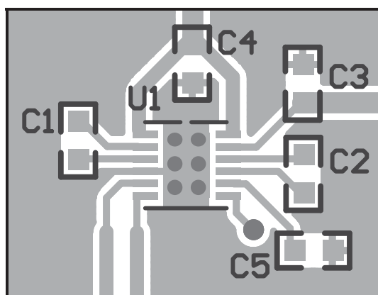
Figure 3: Example PCB Layout.
