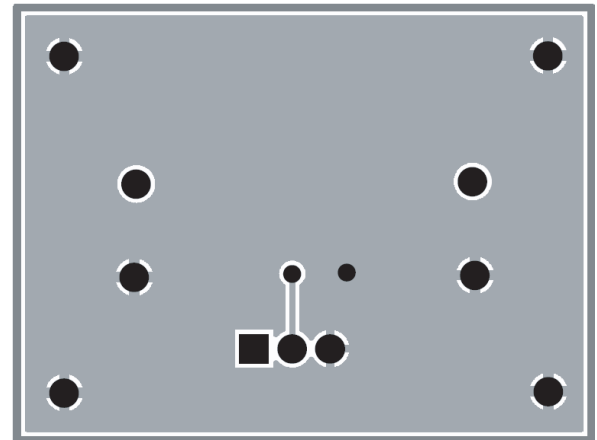
Figure 5: AAT3183 Evaluation Board Bottom Layer
