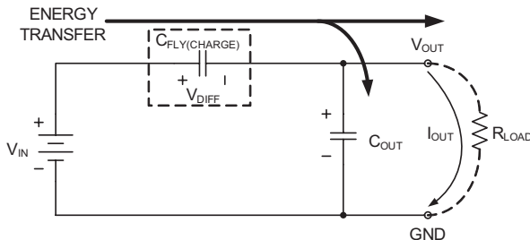
Figure 1a: Step-Down Charge Pump "CHARGE" Interval.
