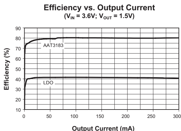
Figure 2: AAT3183 Efficiency Comparison vs. LDO.
