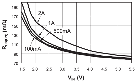
R_{DS(ON)} vs. V_{IN}
