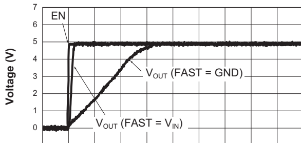
Output Turn-On (R_L = 10\Omega)
