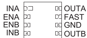
FTDFN22-8 (Top View)
