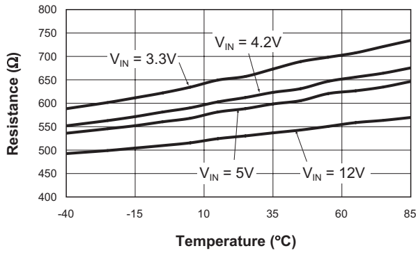
Output Pull-Down Resistance vs. Temperature
