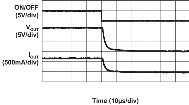
Turn-Off ( V_{IN} = 12\text{V} ; 600mA Load)
