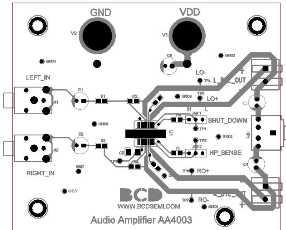
Figure 22. Top Route and Silk Screens
