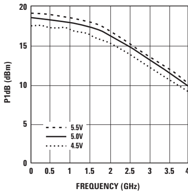
Figure 10. Output Power for 1dB Gain Compression vs. Frequency and Voltage.
