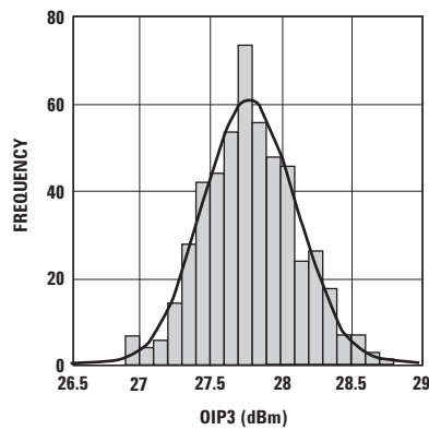
Figure 4. OIP3 Distribution.
