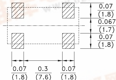
Electrode arrangement
