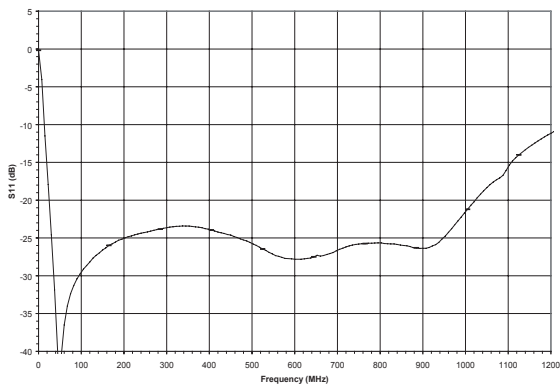
Figure 17: Input Return Loss vs. Frequency ( V_{DD} = +12\text{ V} , I_{DD} = 325\text{ mA} )
