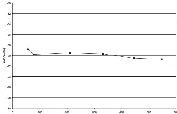
Figure 22: XMOD vs. Frequency ( V_{DD} = +12\text{ V} , I_{DD} = 325\text{ mA} , 79 Analog Channels, 15.6 dB Tilt, +49 dBmV output power at 1 GHz)
