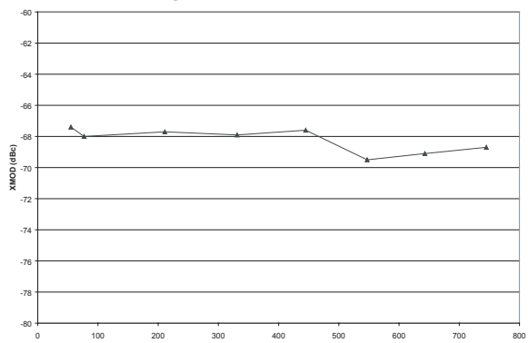
Figure 14: XMOD vs. Frequency ( V_{DD} = +12\text{ V} , I_{DD} = 195\text{ mA} , 112 Analog Channels, 3 dB Tilt, +37 dBmV output power at 1 GHz)
