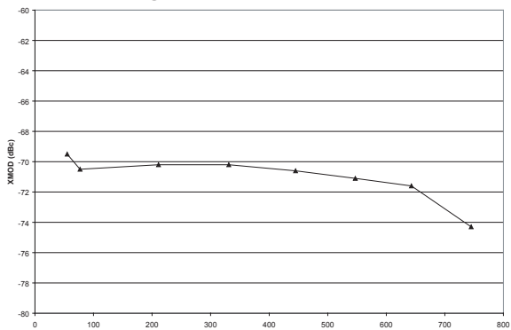
Figure 25: XMOD vs. Frequency
