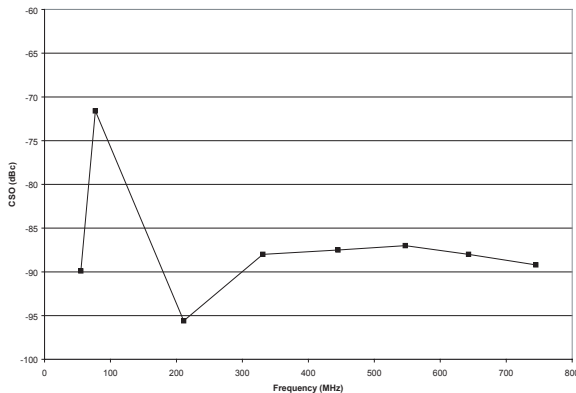
Figure 24: CSO vs. Frequency
