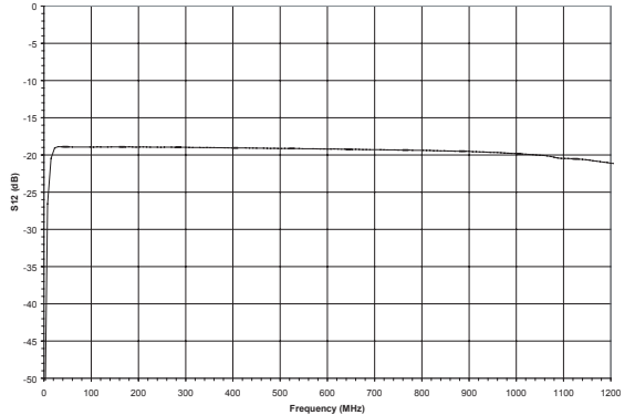
Figure 5: Reverse Isolation vs. Frequency ( V_{DD} = +12\text{ V} , I_{DD} = 195\text{ mA} )
