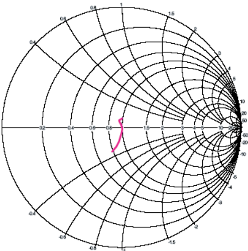
Figure 37. GPS Port Impedance (S44), 1570-1580 MHz.
