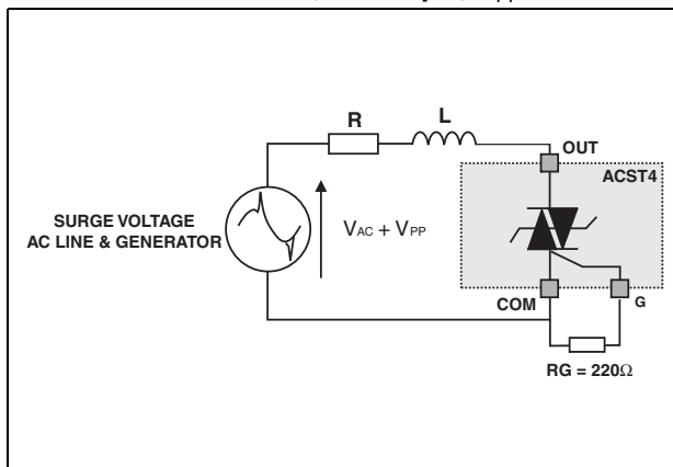
Figure 3. Overvoltage ruggedness test circuit for resistive and inductive loads according to IEC 61000-4-5 standards. R = 150 \Omega , L = 10 \mu\text{H} , V_{PP} = 2 \text{ kV} .
