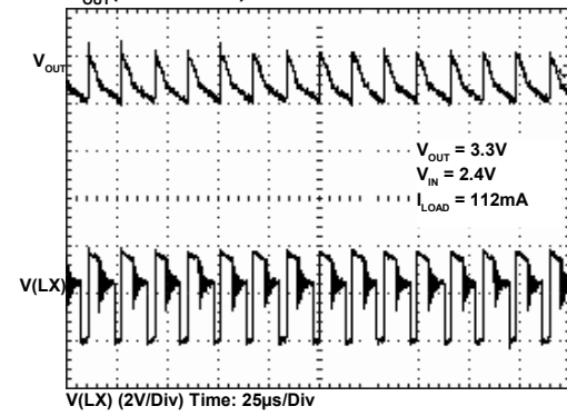
DCM Mode Connection High ESR Output Capacitor V_{OUT} (100mV/Div)
