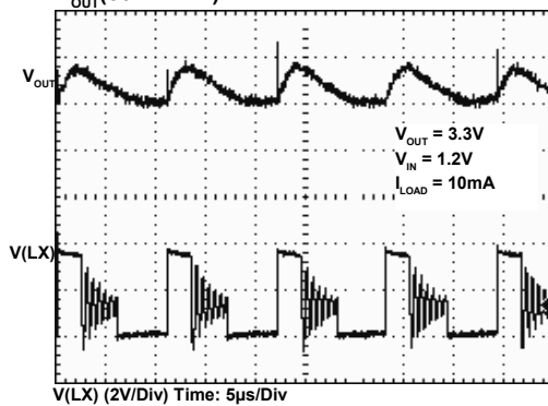
DCM Mode Connection Low ESR Output Capacitor V_{OUT} (50mV/Div)
