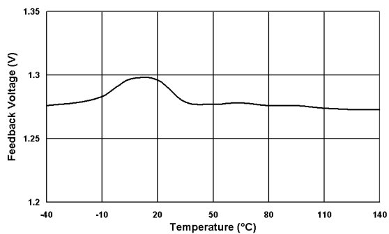
Feedback Voltage vs. Temperature
