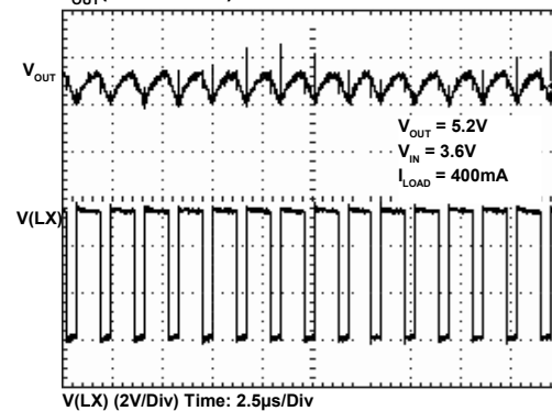
Heavy Load Condition Low ESR Output Capacitor V_{OUT} (100mV/Div)
