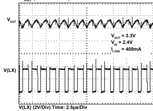
Current Limit Condition Low ESR Output Capacitor V_{OUT} (100mV/Div)
