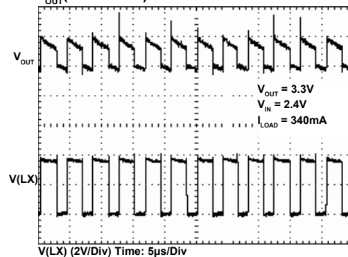
Heavy Load Condition High ESR Output Capacitor V_{OUT} (100mV/Div)
