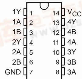
CD54ACT02... F PACKAGE CD74ACT02... E OR M PACKAGE (TOP VIEW)
