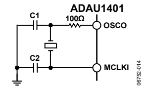
Figure 14. Crystal Oscillator Circuit
