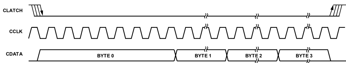
Figure 26. SPI Write to ADAU1401 Clcking (Single-Write Mode)
