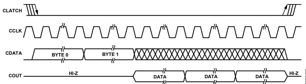
Figure 27. SPI Read from ADAU1401 Clcking (Single-Read Mode)
