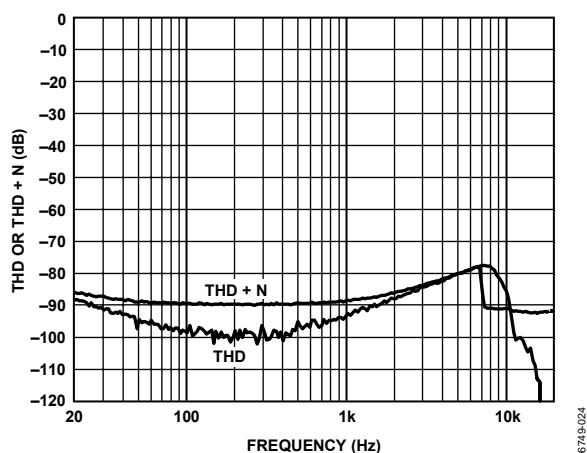
Figure 24. THD or THD + N vs. Frequency @ 1 W, 6 \Omega , PVDD = 15 V, PGA = 0 dB
