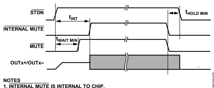
Figure 2. Timing Diagram (Minimum)
