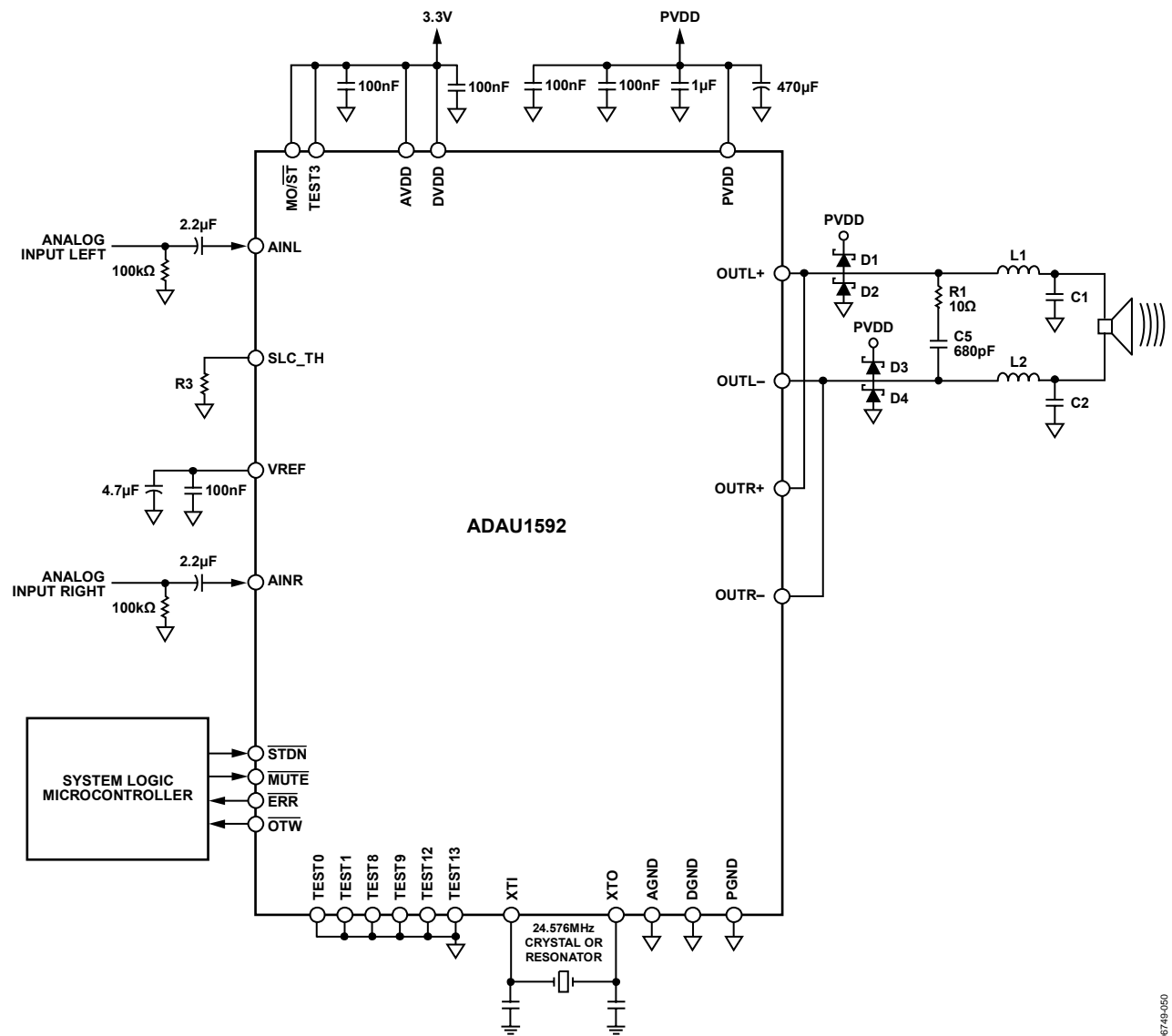
Figure 50. Typical Mono Application Circuit
