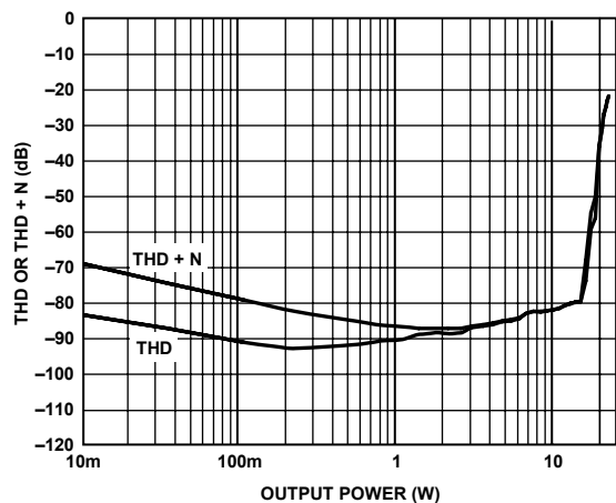
Figure 11. THD or THD + N vs. Output Power, 4 \Omega , PVDD = 15 V
