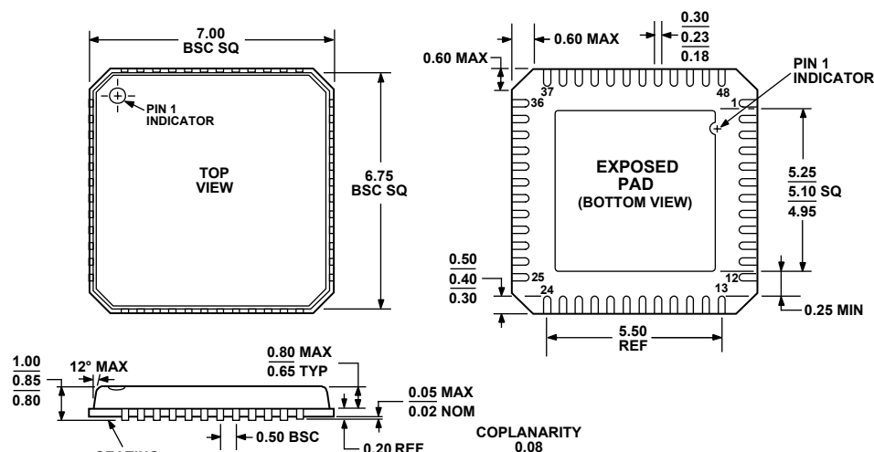
Figure 51. 48-Lead Lead Frame Chip Scale Package [LFCSP_VQ] 7 mm x 7 mm Body, Very Thin Quad (CP-48-1) Dimensions shown in millimeters
