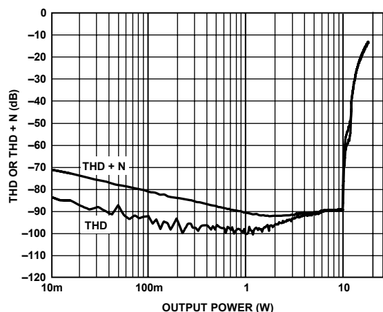
Figure 13. THD or THD + N vs. Output Power, 8 \Omega , PVDD = 15 V
