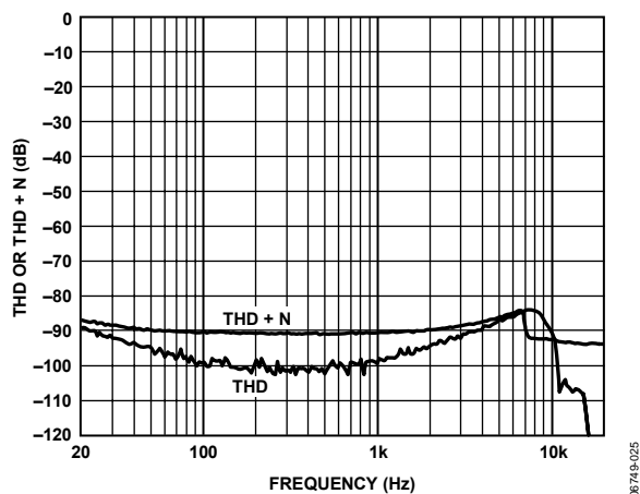
Figure 25. THD or THD + N vs. Frequency @ 1 W, 8 \Omega , PVDD = 15 V, PGA = 0 dB
