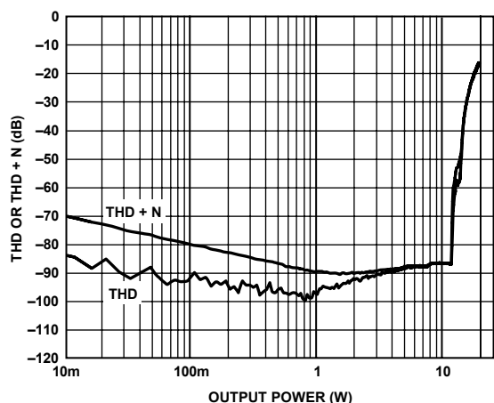
Figure 12. THD or THD + N vs. Output Power, 6 \Omega , PVDD = 15 V
