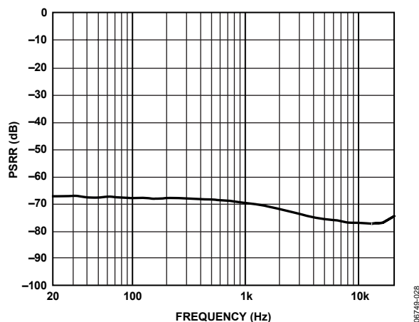
Figure 28. PSRR vs. Frequency, No Input Signal, Ripple = 1.5 V p-p, PVDD = 15 V, 6 \Omega
