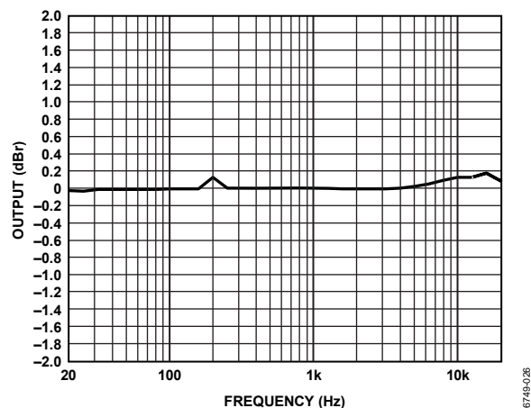
Figure 26. Frequency Response @ 1 W, 6 \Omega , PVDD = 15 V, PGA = 0 dB
