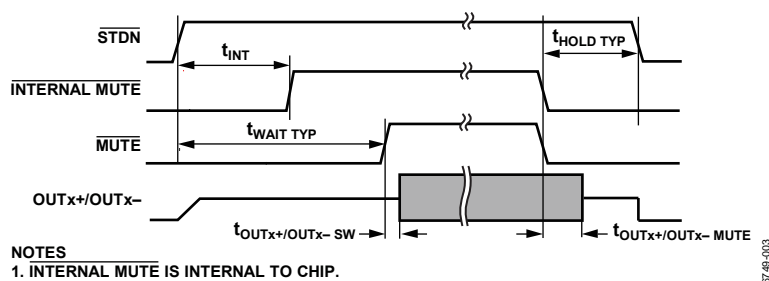
Figure 3. Timing Diagram (Typical)
