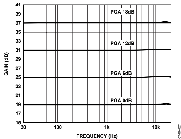
Figure 27. Gain vs. Frequency @ 1 W, 6 \Omega , PVDD = 15 V
