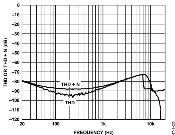
Figure 23. THD or THD + N vs. Frequency @ 1 W, 4 \Omega , PVDD = 15 V, PGA = 0 dB
