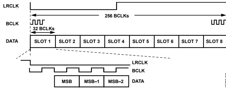
Figure 34. TDM Mode
