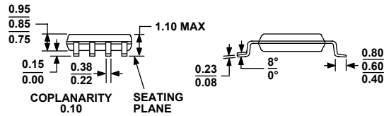
Figure 37. 8-Lead Mini Small Outline Package [MSOP] (RM-8)
