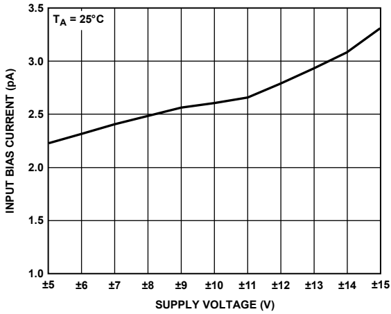
Figure 19. Input Bias Current vs. Supply Voltage
