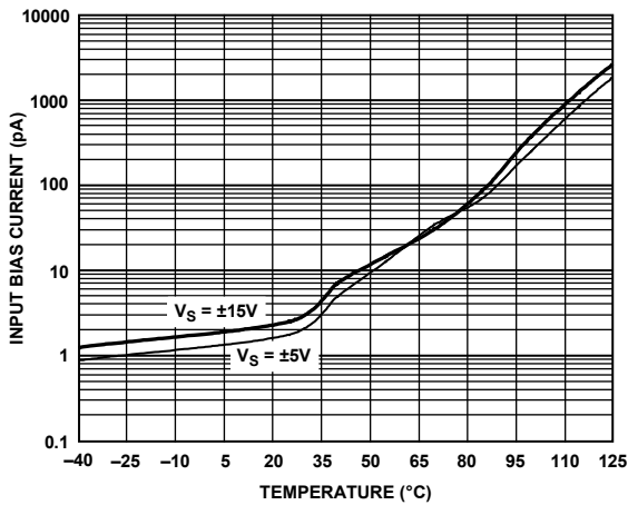
Figure 20. Input Bias Current vs. Temperature
