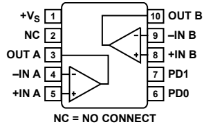
Figure 5. 10-Lead MSOP Pin Configuration
