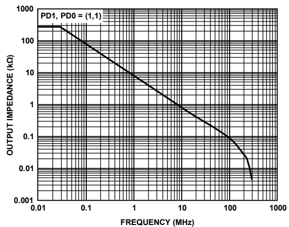
Figure 17. Output Impedance vs. Frequency (Disabled)
