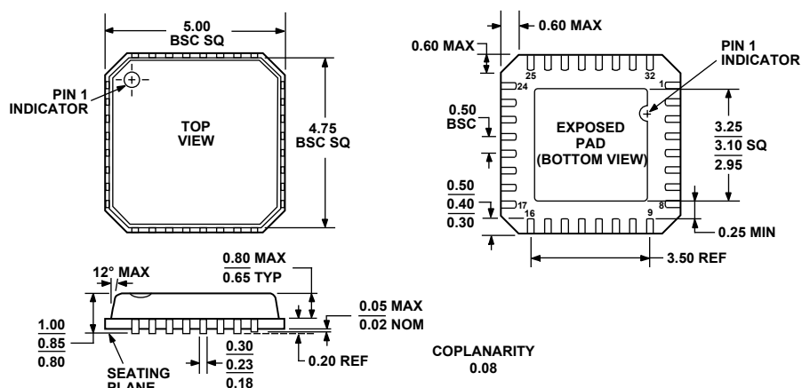
Figure 28. 32-Lead Lead Frame Chip Scale Package [LFCSP_VQ]
