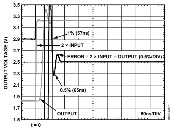
Figure 18. Settling Time
