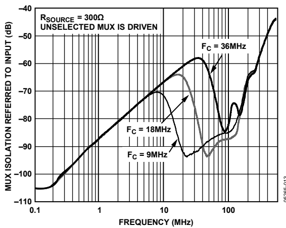
Figure 12. HD Mux Isolation vs. Frequency and Cutoff Frequency
