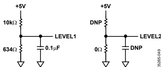
Figure 24. Flexible Circuits to Set the LEVEL1 and LEVEL2 Inputs to Obtain a 600 mV Output Offset on a Single Supply ( G = \times 2 )
