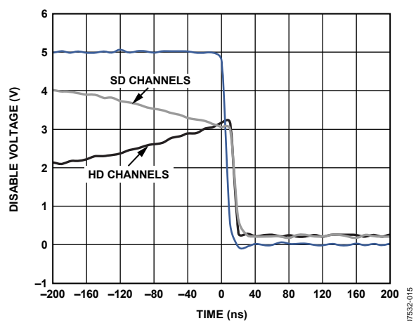
Figure 15. Disable Turn-Off Time
