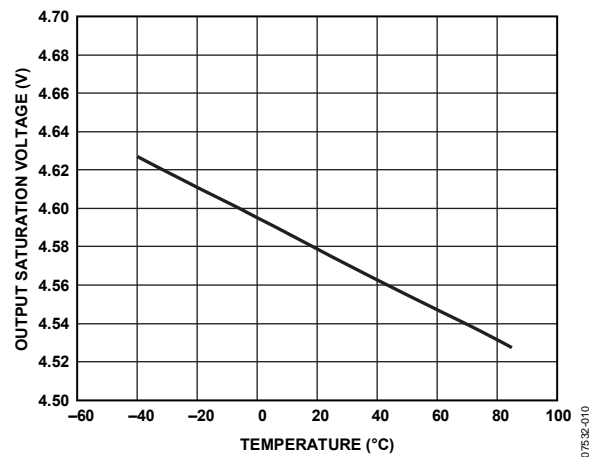
Figure 16. Output Saturation Voltage vs. Temperature
