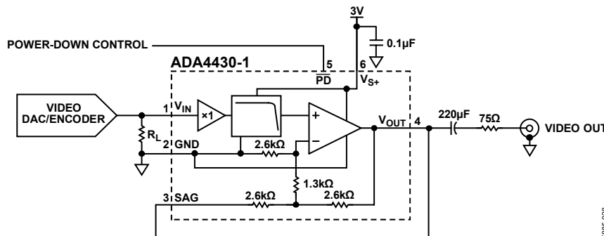
Figure 30. Traditional AC-Coupled Output with 220 µF Coupling Capacitor
