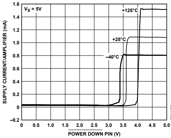
Figure 31. Supply Current per Amplifier vs. POWER DOWN Pin Voltage
