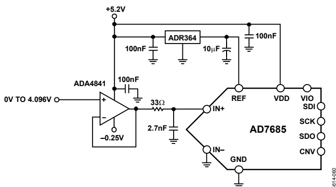
Figure 49. ADC Driver Schematic
