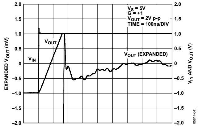
Figure 28. Settling Time
