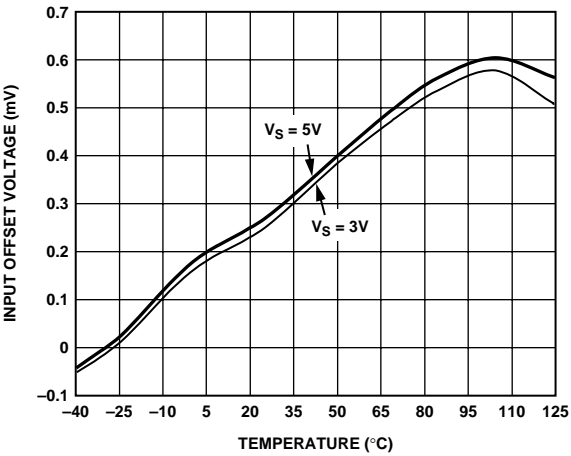
Figure 36. Input Offset Voltage vs. Temperature for Various Supplies
