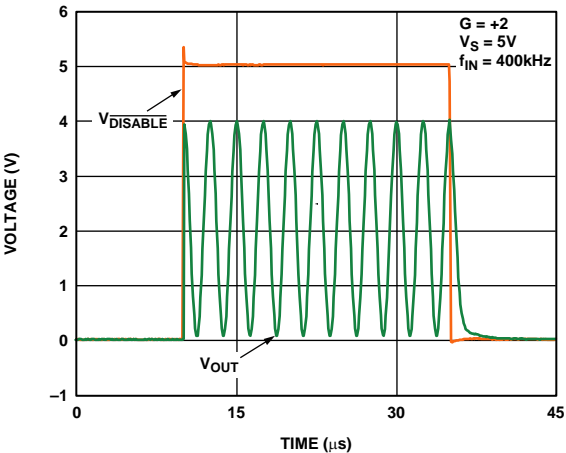
Figure 23. Enable/Disable Time
