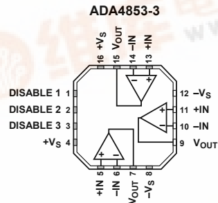
Figure 3. 16-Lead LFCSP_VQ
