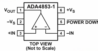
Figure 1. 6-Lead SC70
