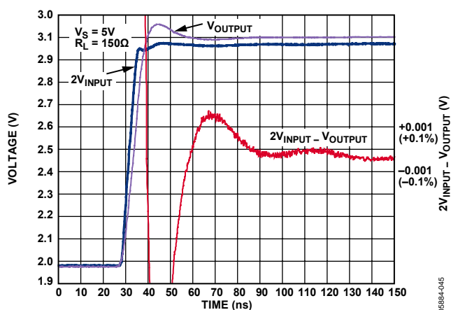
Figure 46. 0.1% Settling Time
