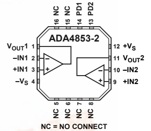
Figure 2. 16-Lead LFCSP_VQ
