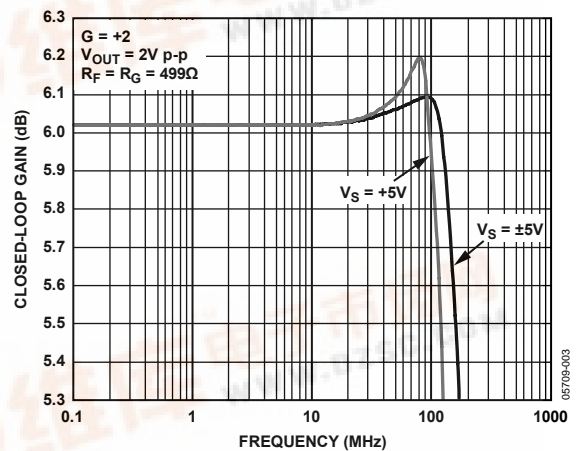
Figure 2. 0.1 dB Flatness
