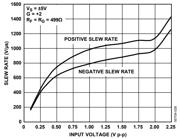
Figure 37. Slew Rate vs. Input Voltage
