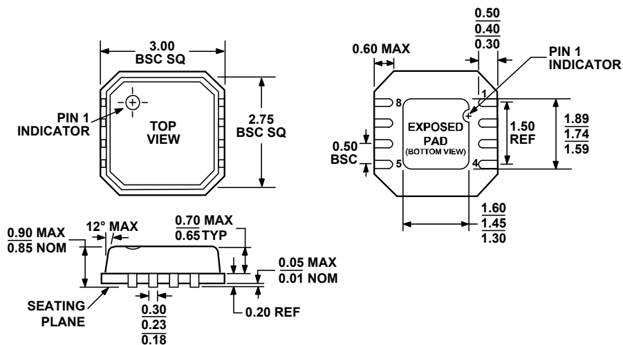
Figure 54. 8-Lead Lead Frame Chip Scale Package [LFCSP_VD] 3 mm \times 3 mm Body, Very Thin, Dual Lead (CP-8-2)
