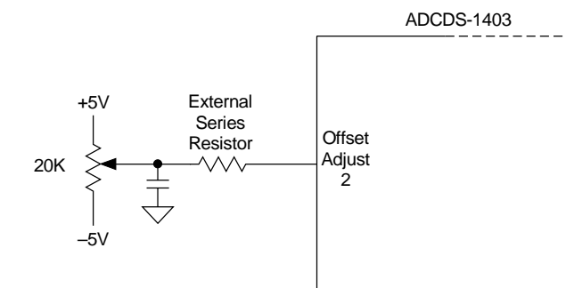
Figure 3. Offset Adjustment Circuit
