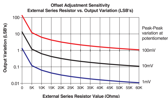
Figure 7. Offset Adjustment Sensitivity
