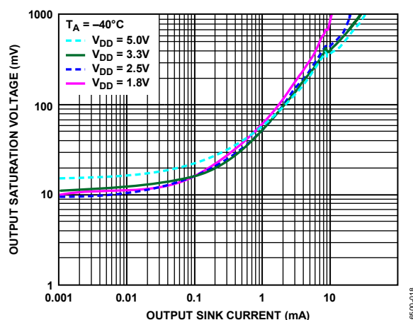
Figure 21. Output Saturation Voltage vs. Output Sink Current
