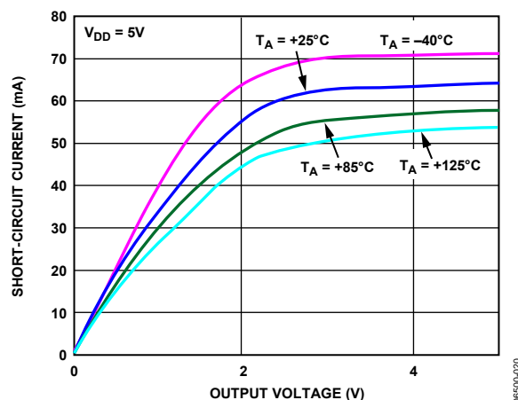
Figure 22. Short-Circuit Current vs. Output Voltage
