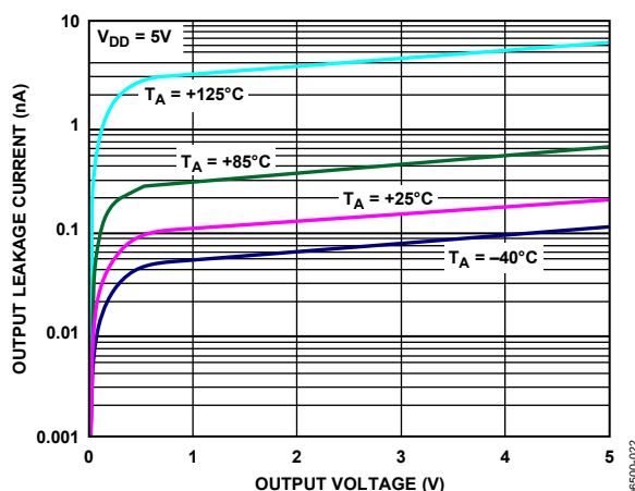
Figure 23. Output Leakage Current vs. Output Voltage
