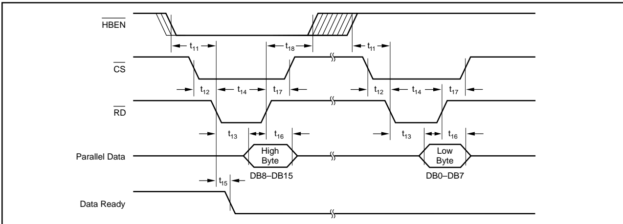
ADC700 Parallel Output Timing.
