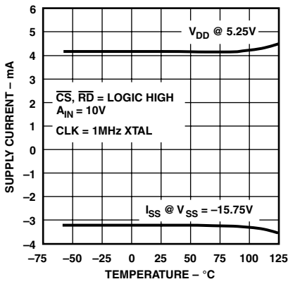
TPC 4. Supply Current vs. Temperature
