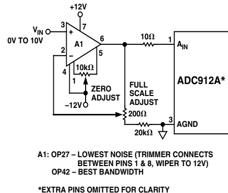
Figure 16. Unipolar 0 V to 10 V Operation
