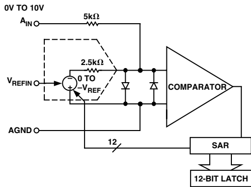
Figure 11. Simplified Analog Input Circuitry of ADC912A
