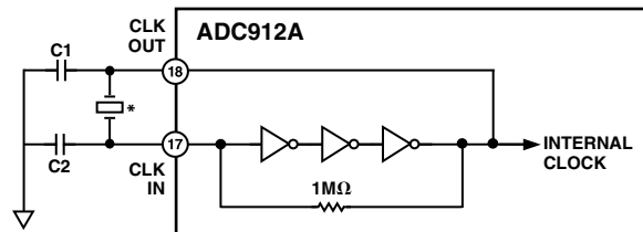
*CRYSTAL OR CERAMIC RESONATOR
