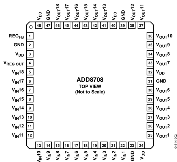
Figure 2. Pin Configuration
