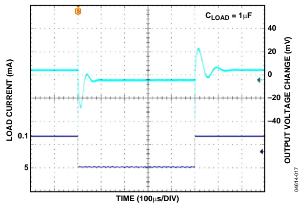
Figure 17. Regulator Load Transient Response
