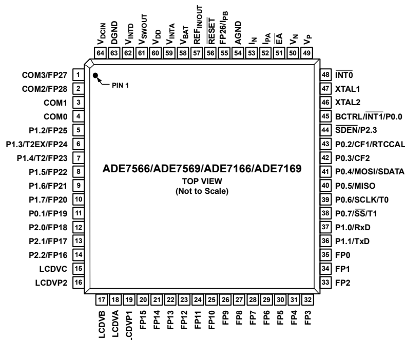
Figure 9. Pin Configuration
