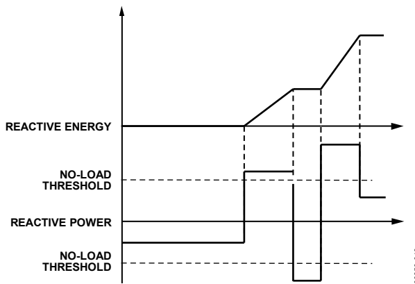
Figure 73. Reactive Energy Accumulation in Absolute Accumulation Mode
