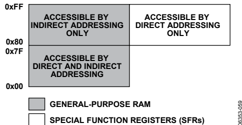
Figure 83. General-Purpose RAM and SFR Memory Address Overlap
