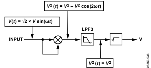
Figure 59. RMS Signal Processing
