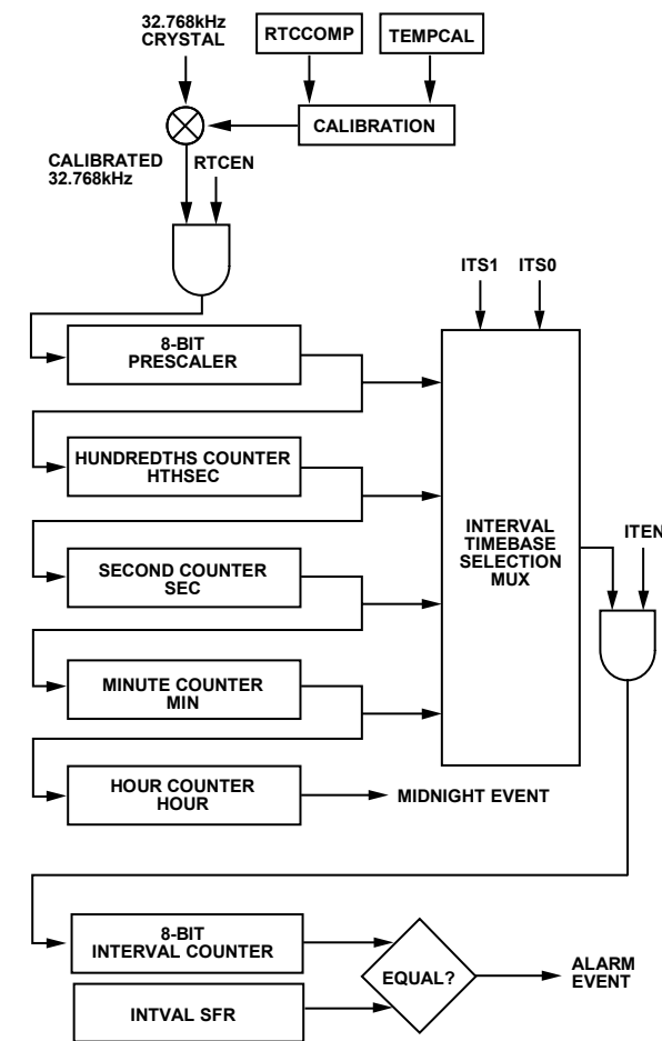
Figure 101. RTC Implementation
