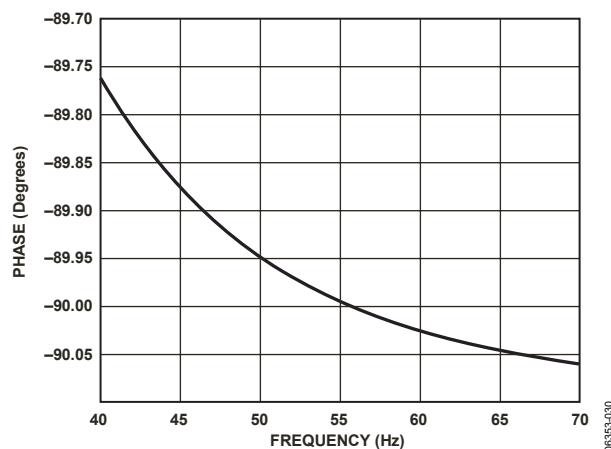
Figure 53. Combined Phase Response of the Digital Integrator and Phase Compensator (40 Hz to 70 Hz)
