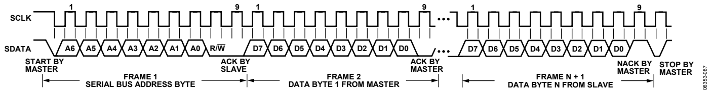
Figure 111. I 2 C Read Operation
