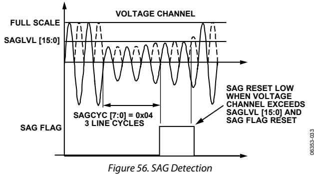
Figure 56. SAG Detection
