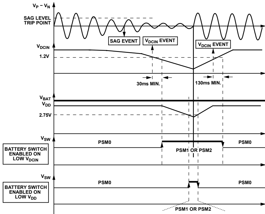
Figure 36. Power Supply Management Transitions Between Modes
