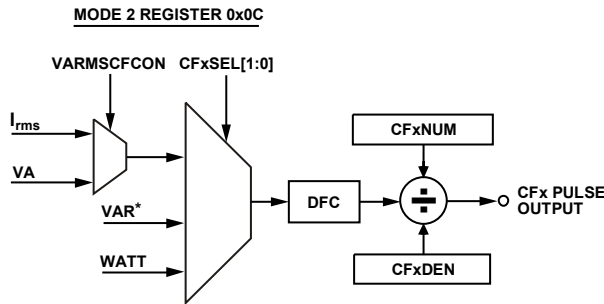
Figure 78. Energy-to-Frequency Conversion
