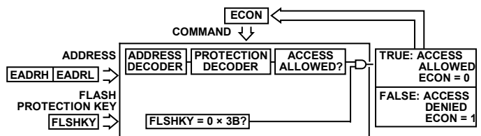
Figure 93. Flash Memory Read/Write/Erase Protection Block Diagram
