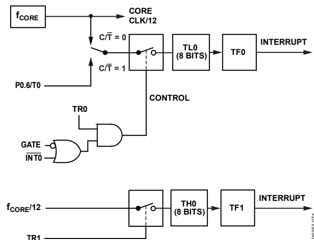
Figure 98. Timer/Counter 0, Mode 3
