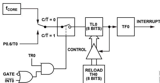
Figure 97. Timer/Counter 0, Mode 2
