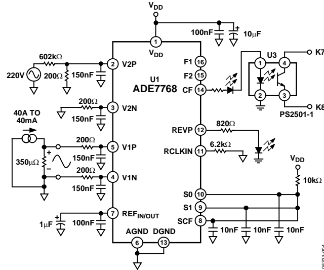
Figure 4. Test Circuit for Performance Curves
