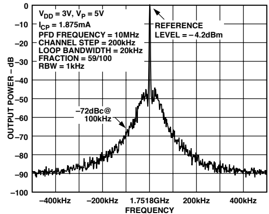
TPC 6. Spurious Plot, Lowest Spur Mode, 1.7518 GHz RF_{OUT} , 10 MHz PFD Frequency, 200 kHz Channel Step Resolution
