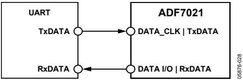
Figure 30. UART to ADF7021 Connection Diagram
