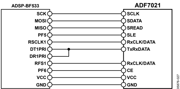
Figure 29. ADSP-BF533 to ADF7021 Connection Diagram
