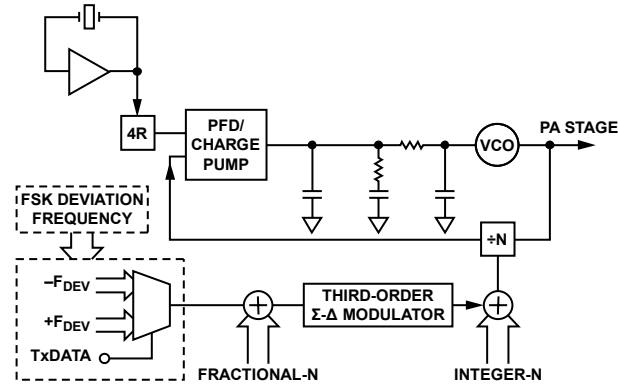
Figure 16. 2FSK Implementation
