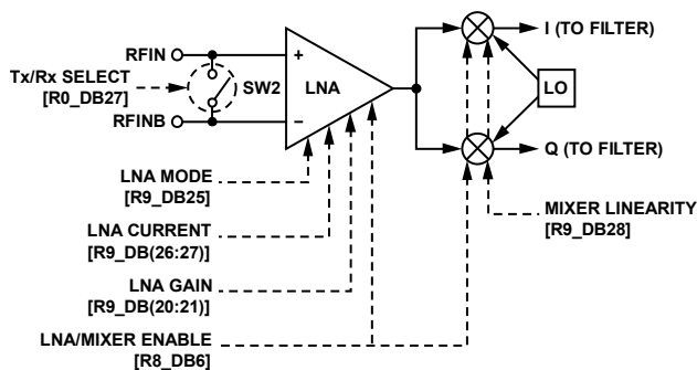
Figure 19. ADF7021 RF Front End
