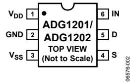
Figure 2. SOT-23 Pin Configuration
