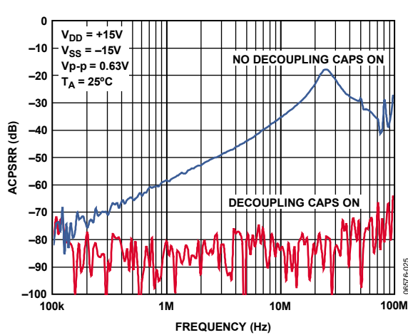
Figure 19. ACPSRR vs. Frequency
