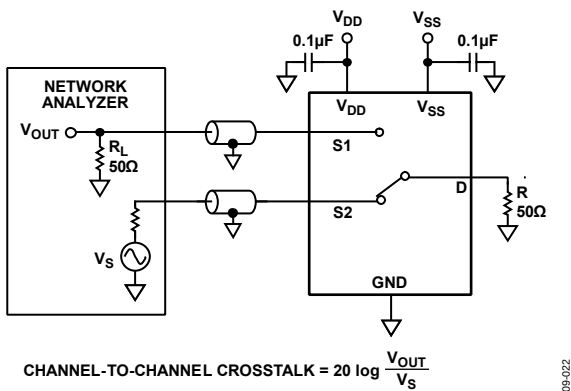
Figure 21. Channel-to-Channel Crosstalk
