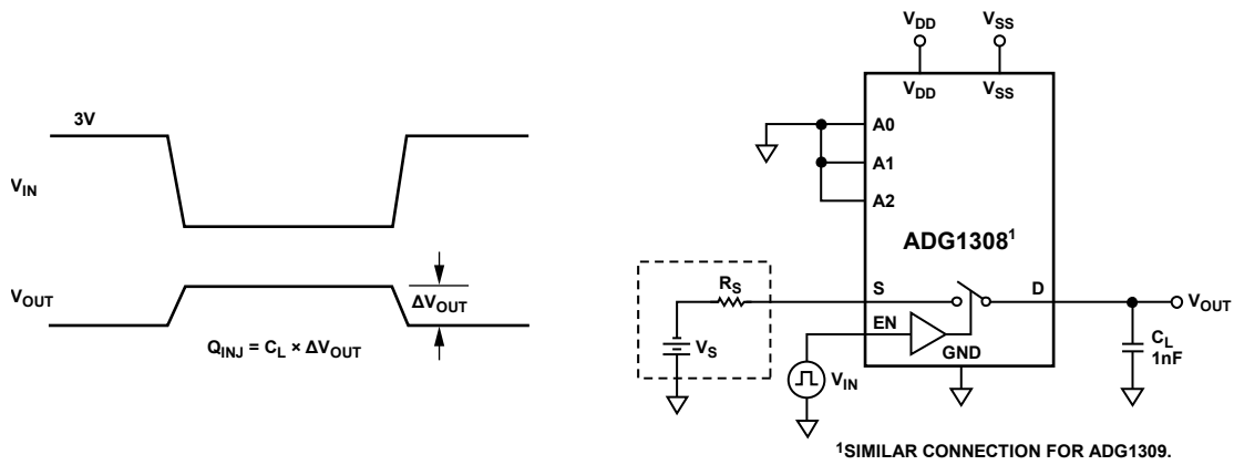
Figure 19. Charge Injection
