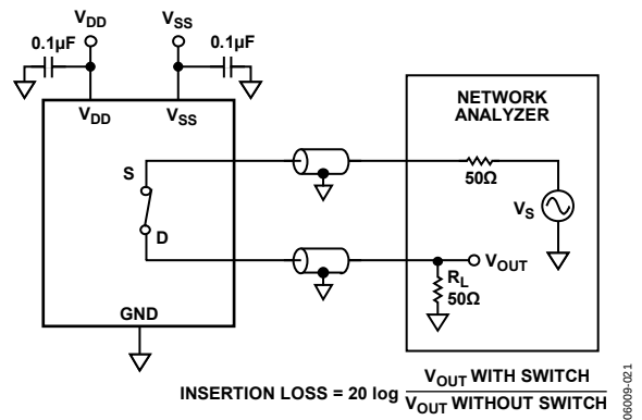
Figure 22. Bandwidth
