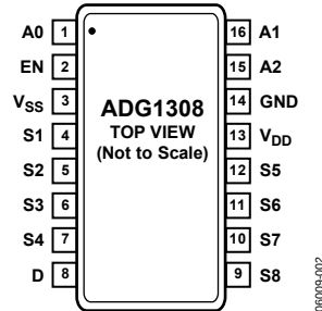
Figure 2. ADG1308 Pin Configuration (TSSOP and SOIC_N)
