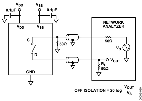
Figure 20. Off Isolation
