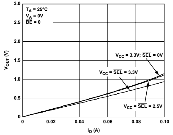
Figure 13. Output Low Characteristic
