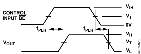
Figure 26. Propagation Delay
