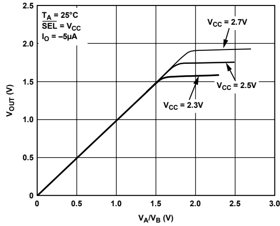
Figure 10. Pass Voltage vs. V_{CC}
