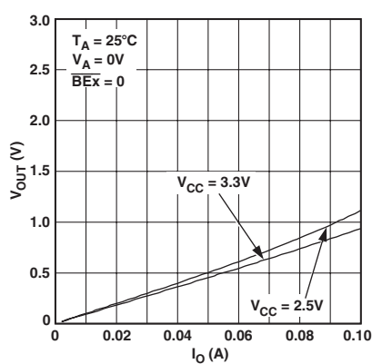
TPC 8. Output Low Characteristic
