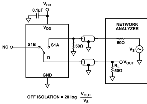
Figure 25. Off Isolation
