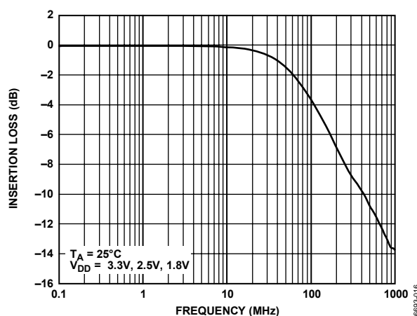
Figure 14. Bandwidth
