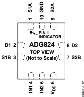
Figure 2. Pin Configuration
