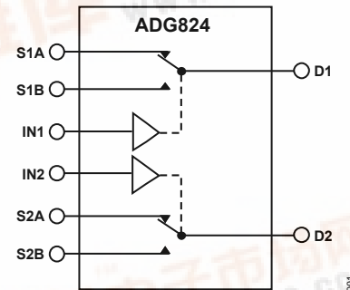
SWITCHES SHOWN FOR A LOGIC 1 INPUT
