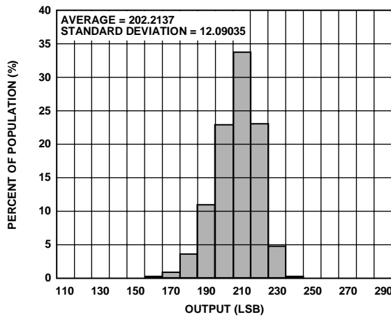
Figure 14. X-Axis Self-Test at 25^\circ\text{C} , V_{CC} = 5\text{ V}
