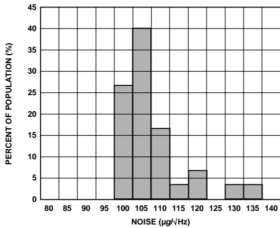
Figure 13. Noise (Y-Axis) at V_{CC} = 5\text{ V} , 25^\circ\text{C}
