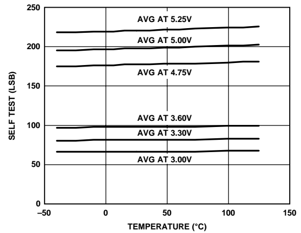
Figure 16. Self-Test X-Axis vs. Temperature
