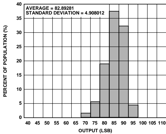
Figure 15. X-Axis Self-Test at 25^\circ\text{C} , V_{CC} = 3.3\text{ V}
