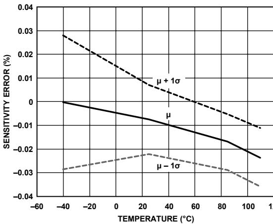
Figure 8. Sensitivity Drift vs. Temperature, V_{CC} = 5\text{ V}
