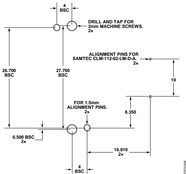
Figure 14. Typical Hole Pattern for the ADIS16365 Attachment
