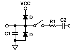
Figure 17. Equivalent Analog Input Circuit Conversion Phase: Switch Open Track Phase: Switch Closed
