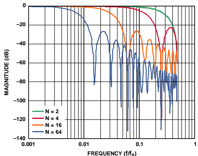
Figure 16. Bartlett Window FIR Frequency Response
