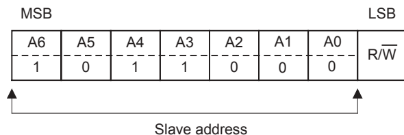
Figure 7. Slave Addressing
