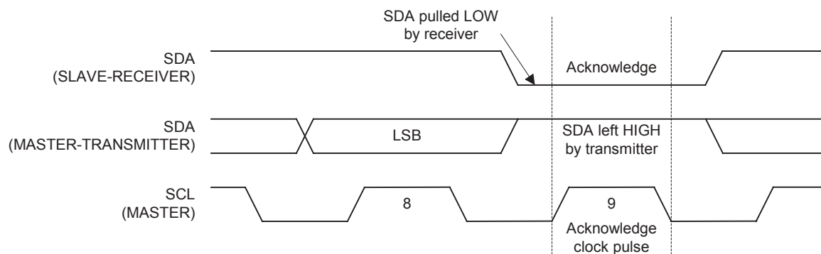
Figure 5. Slave-Receiver Acknowledge
