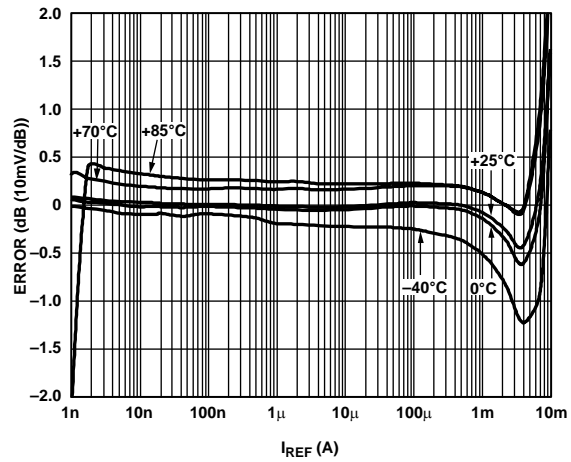
Figure 7. Law Conformance Error vs. I_{REF} for Multiple Temperatures, Normalized to 25°C ( I_{INP} = 3 \mu A )
