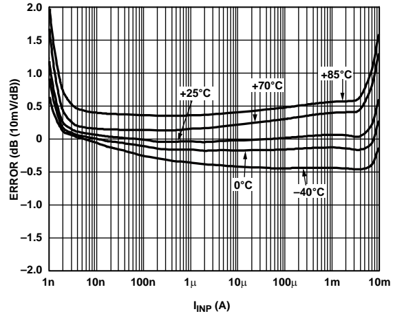
Figure 6. Law Conformance Error vs. I_{INP} for Multiple Temperatures, Normalized to 25°C
